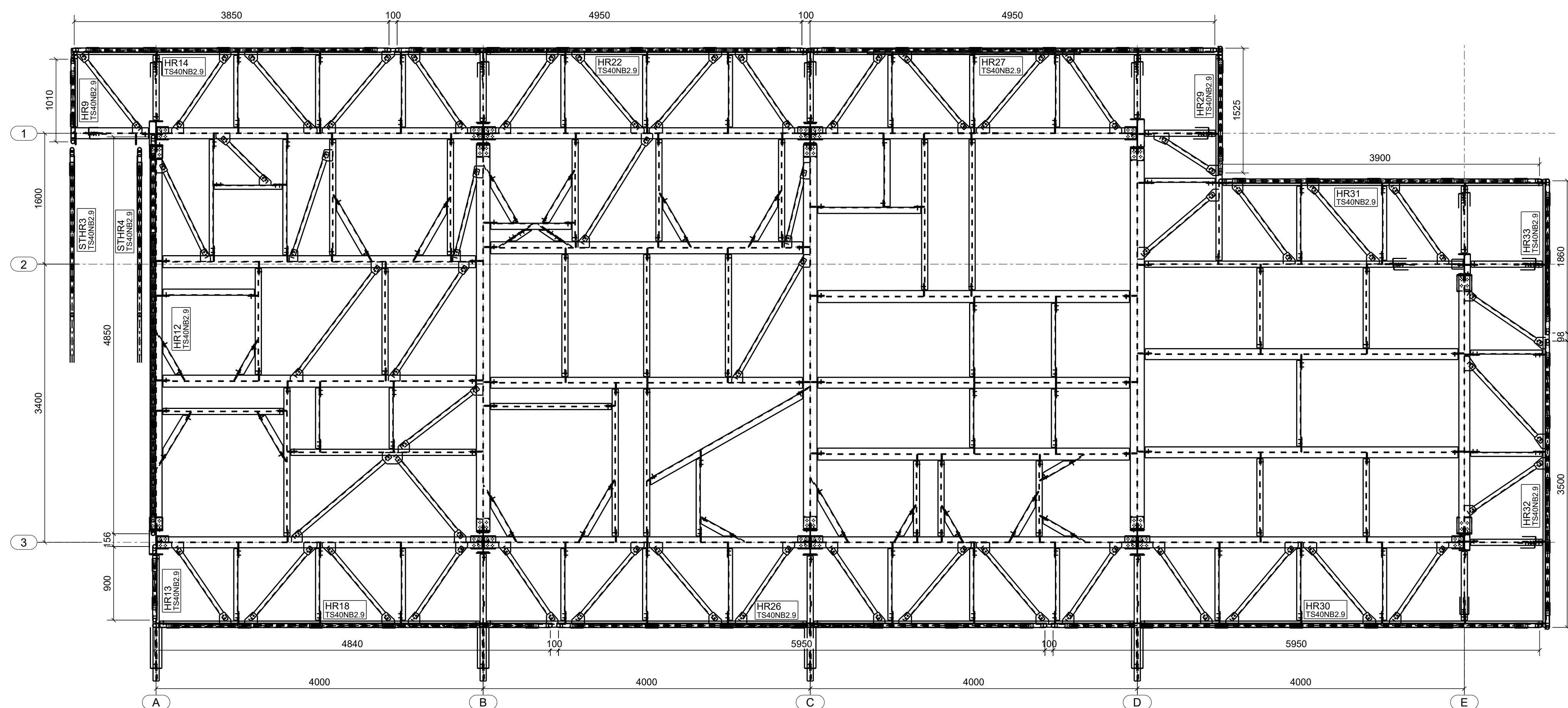
MARKING PLAN FOR HANDRAIL AT EL.+11.000 LVL. SCALE :- 1:35
