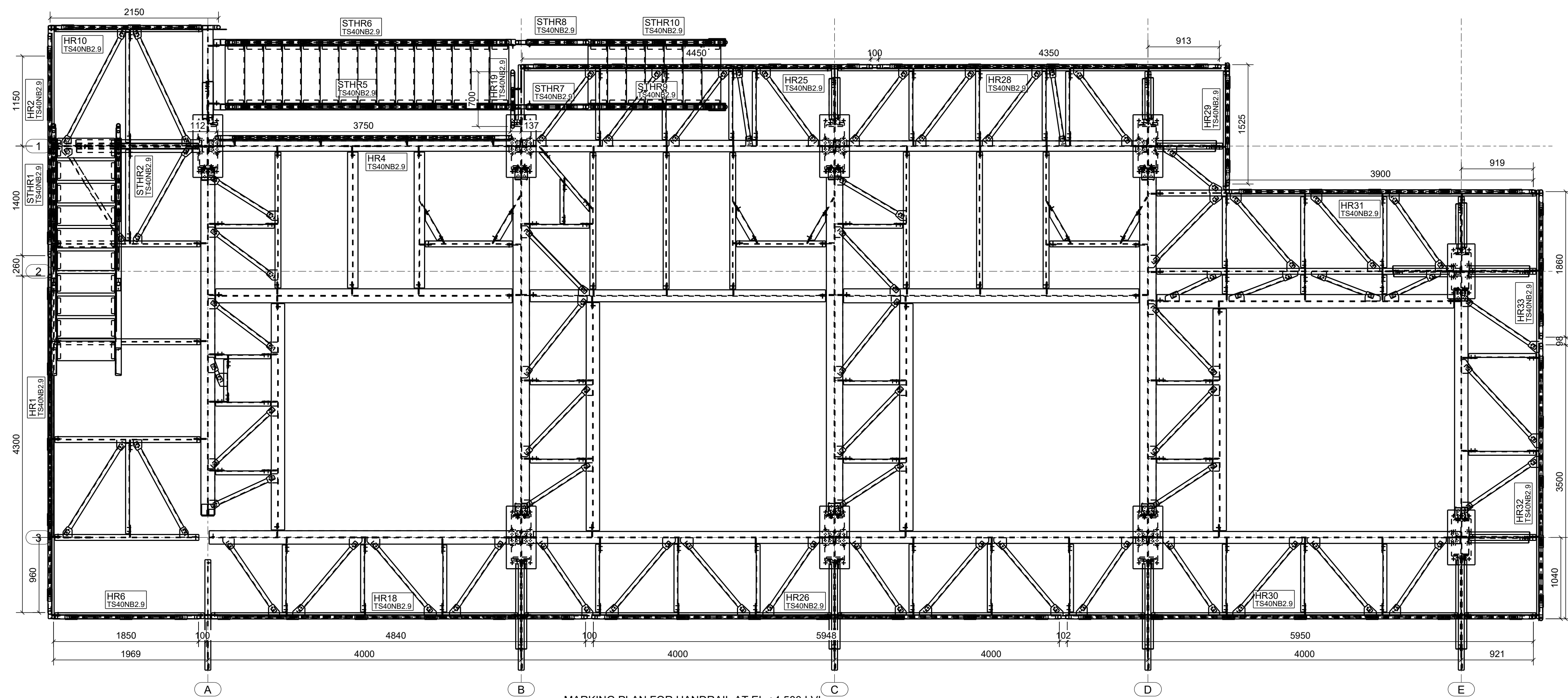
MARKING PLAN FOR HANDRAIL AT EL.+4.500 LVL. SCALE - 1:35
