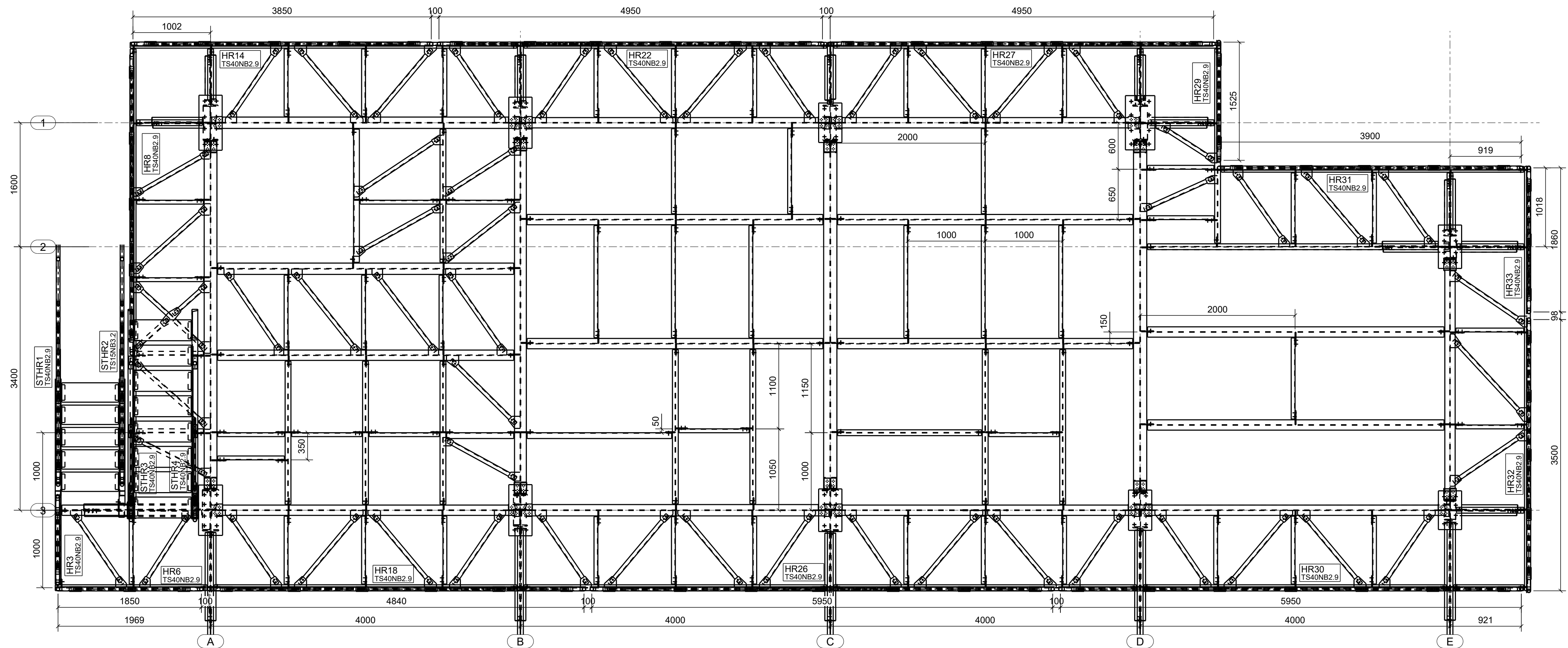
MARKING PLAN FOR HANDRAIL AT EL.+8.000 LVL. SCALE - 1:35
